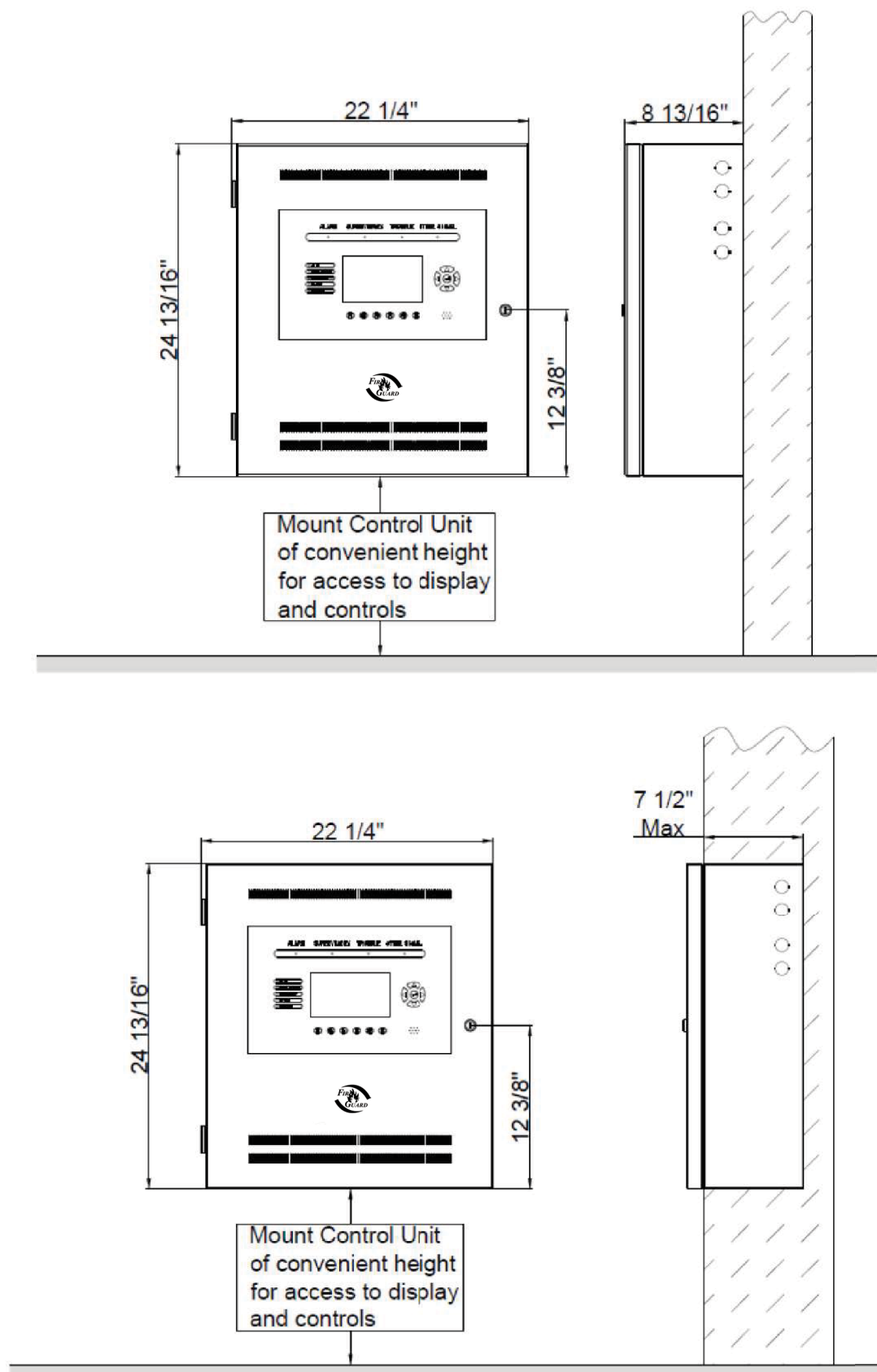
Figure iQ600 Enclosure Mounting Size
